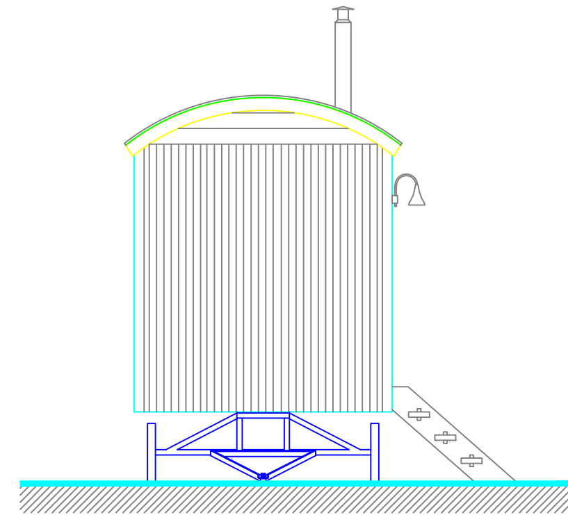
Left elevation
